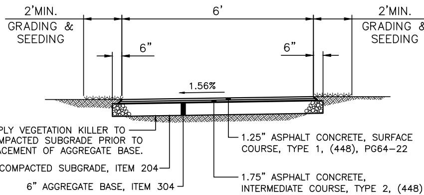
MULTI-USE PATH DETAIL No Scale
